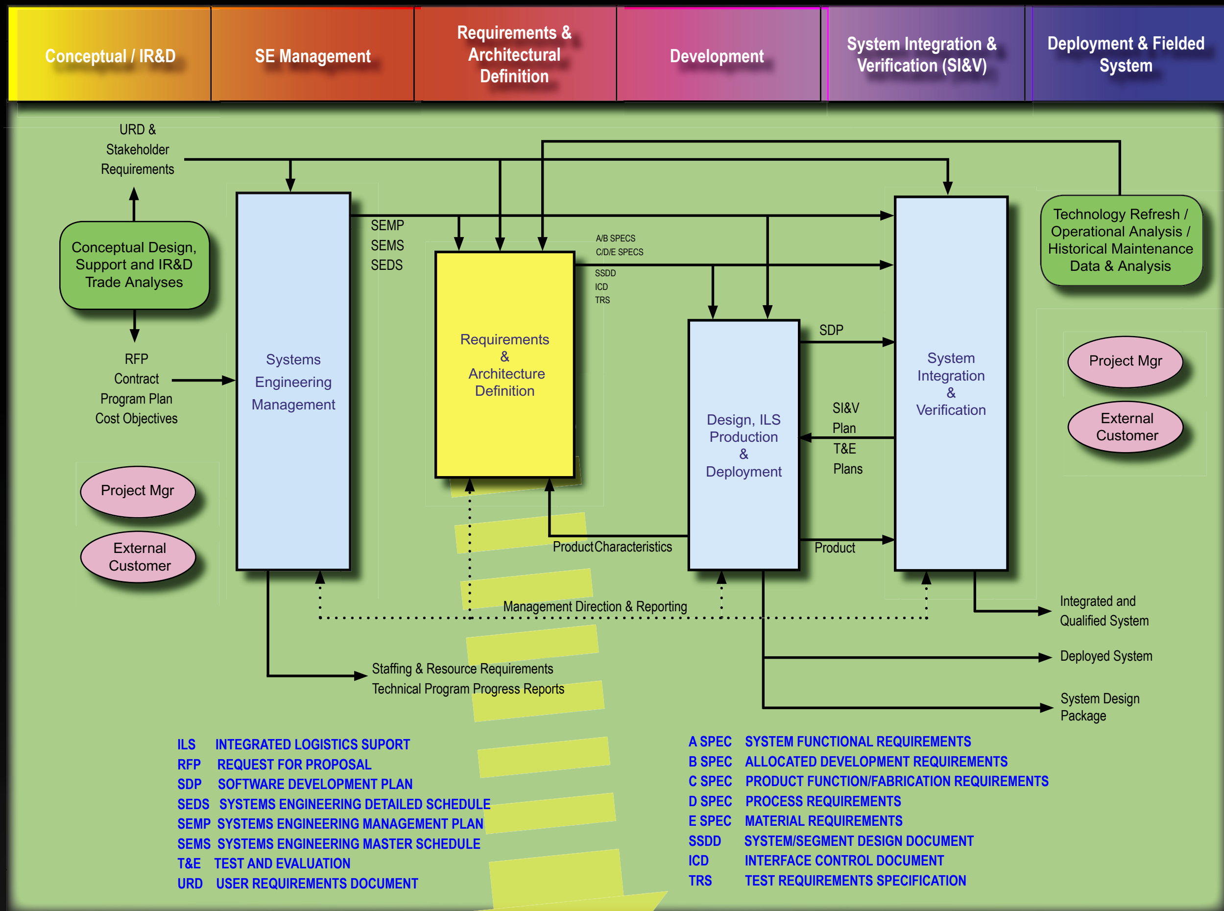
Systems Engineering Process Overview
